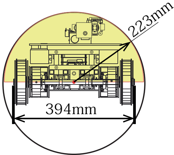
Fig. 7. Sectional View of sub-crawler
