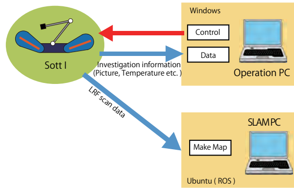
Fig. 16. system configuration
