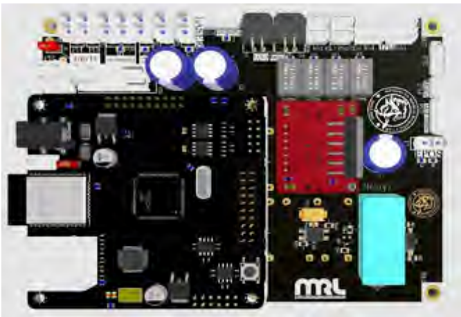
Fig. 8. ARM-based main controller.
