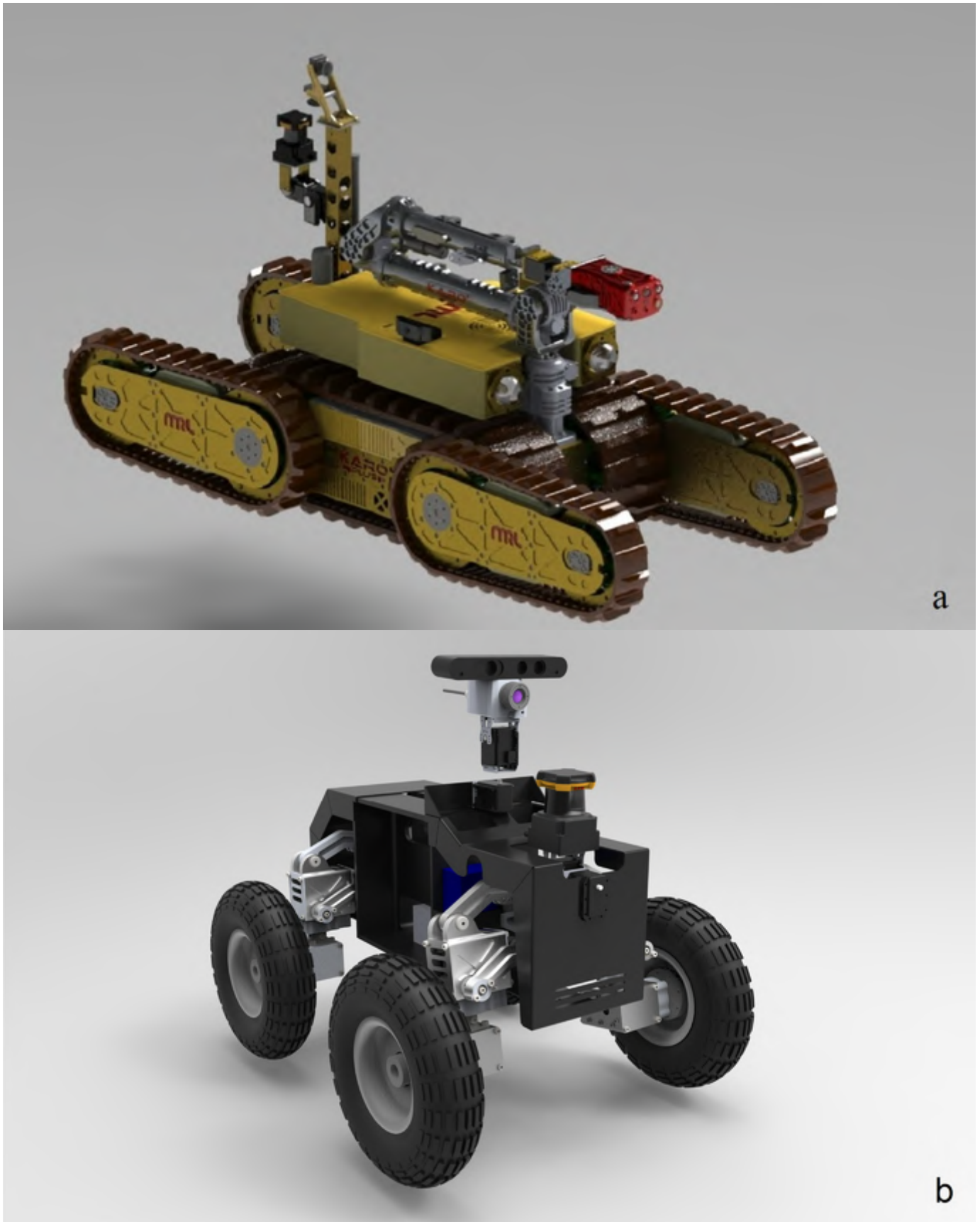
Fig. 19. a: CAD drawing of Karo Plus and the 6-DOF manipulator. b: CAD drawing of Adrina, the autonomous rescue robot.
