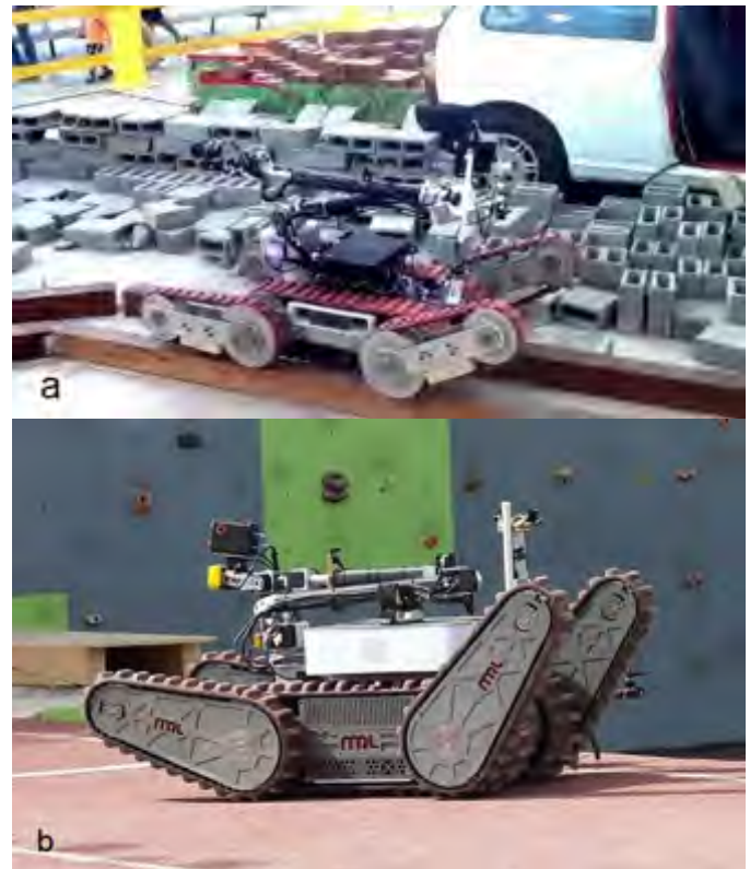
Fig. 6. a: Ario in Robocup Rescue 2014, Brazil. b: Karo in Qazvin firefighter's training camp, Iran.
