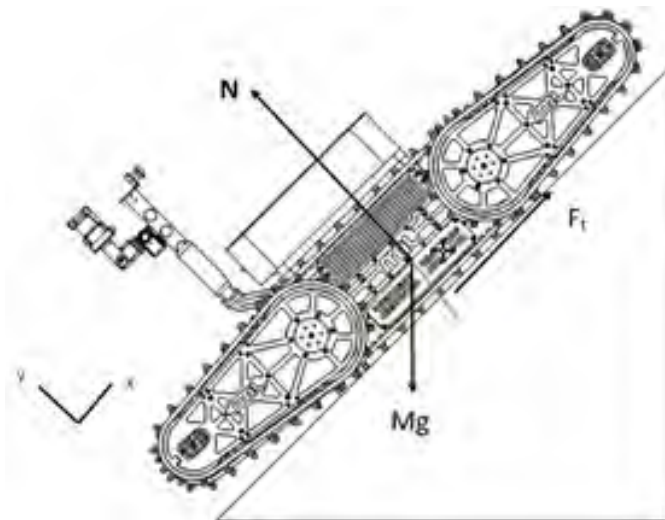
Fig. 12. Free body diagram of the robot on the slope.
