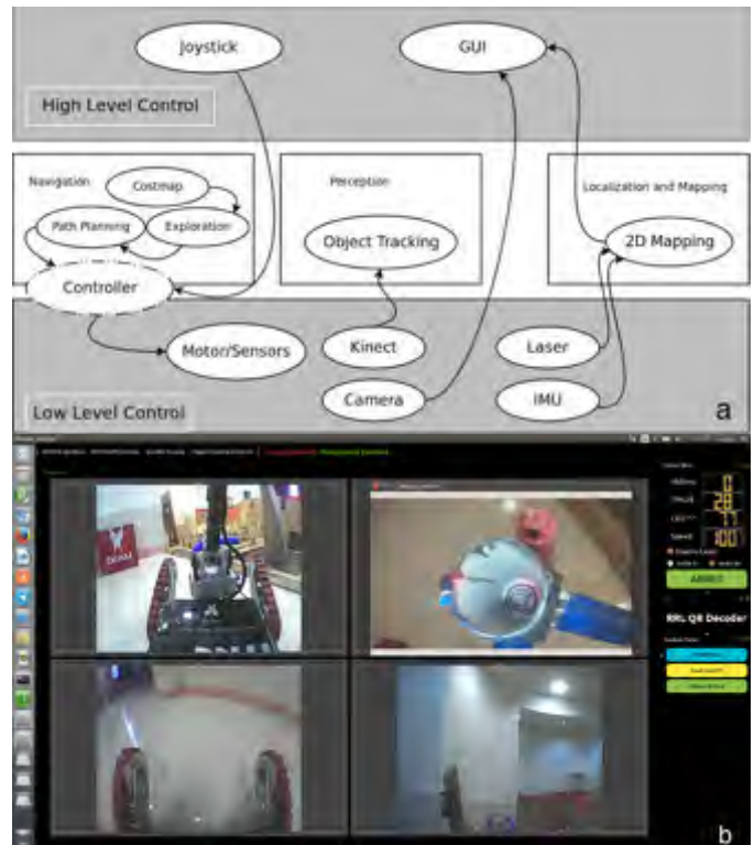
Fig. 15. a: Software system block diagram. b: GUI of human-robot interface.
