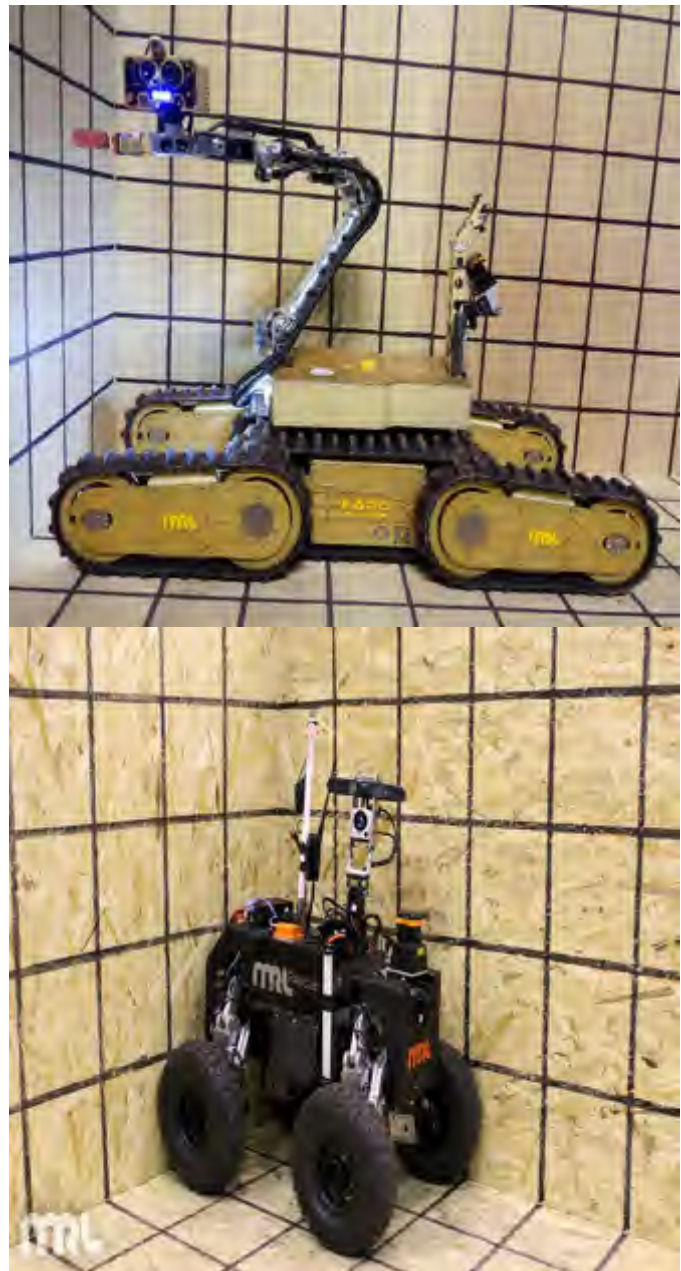
Fig. 1. Karo Plus, a track tele-operative rescue robot, in Robocup Rescue 2016, Germany and Adrina, an autonomous rescue robot, in Robocup Rescue 2015, China.
