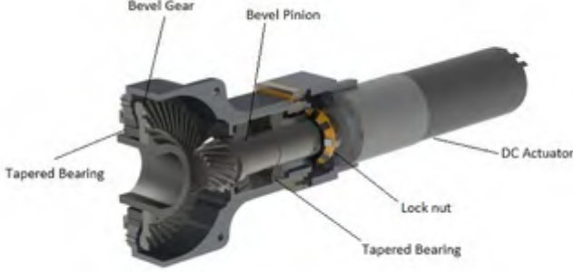
Fig. 13. Bevel gearbox assembly of Karo.
