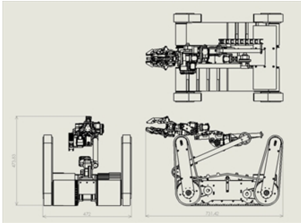
Fig. 9. CAD Drawing of R-5 with arm mounted
