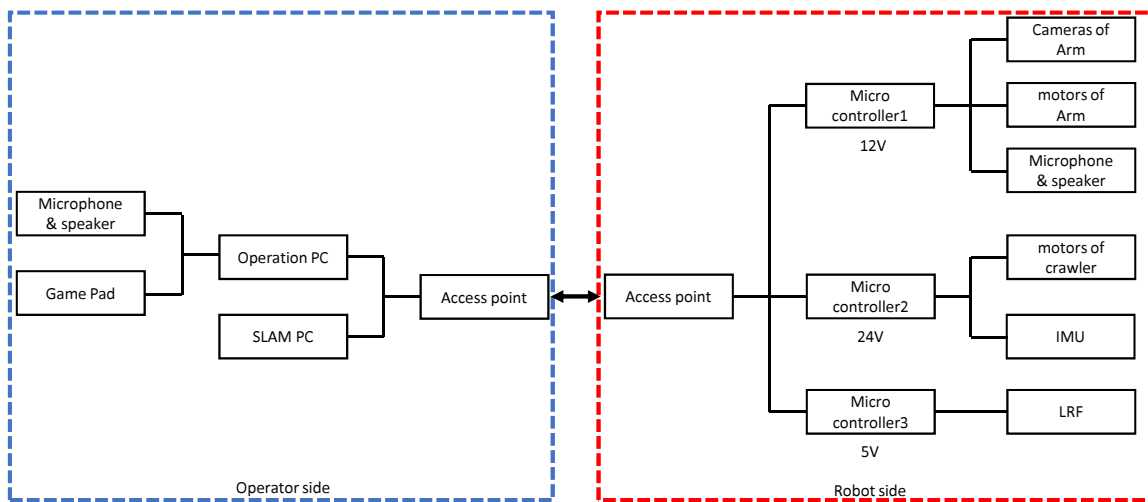
Fig. 5. Control system diagram of R5
