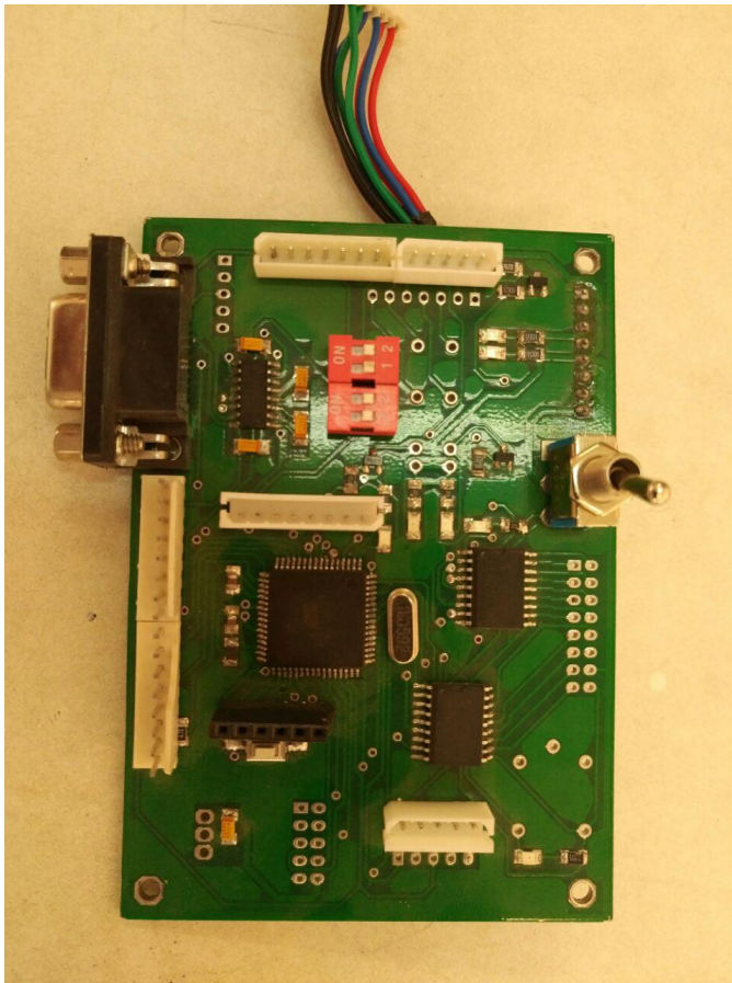
Fig. 4. Microcontroller Board
