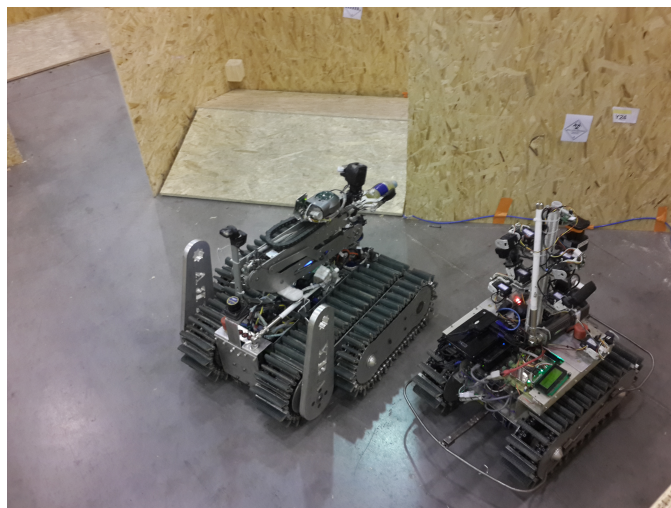
Fig. 6. Autonomous and Tele operation Robots
