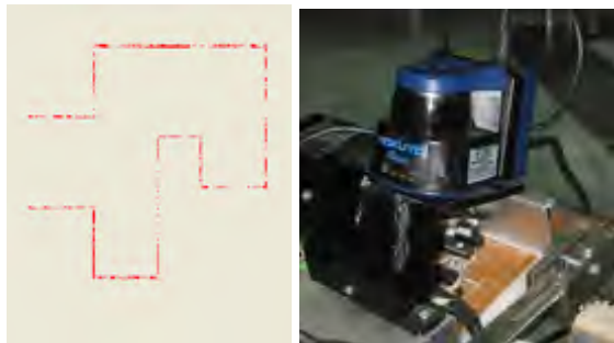
Fig 8 laser scanner (Hokuyo UGB-04LX-F01)
