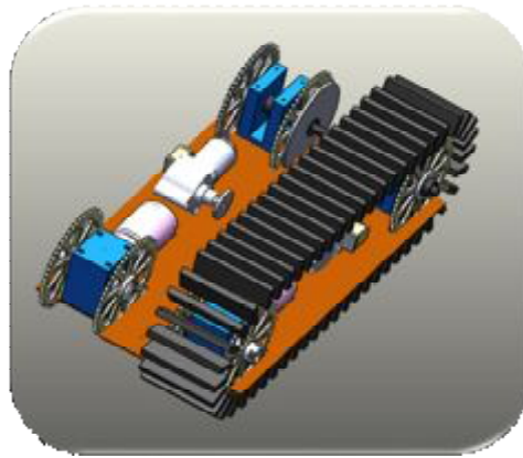
Fig. 7. Motors and straps
