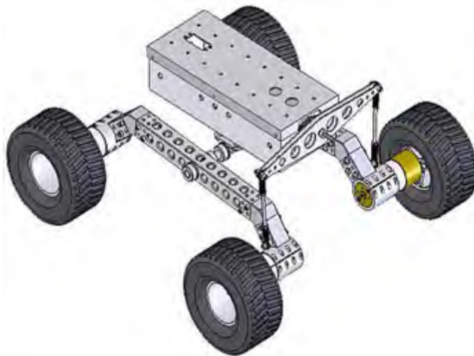
Fig. 15 The basic platform of the Gears SMP
