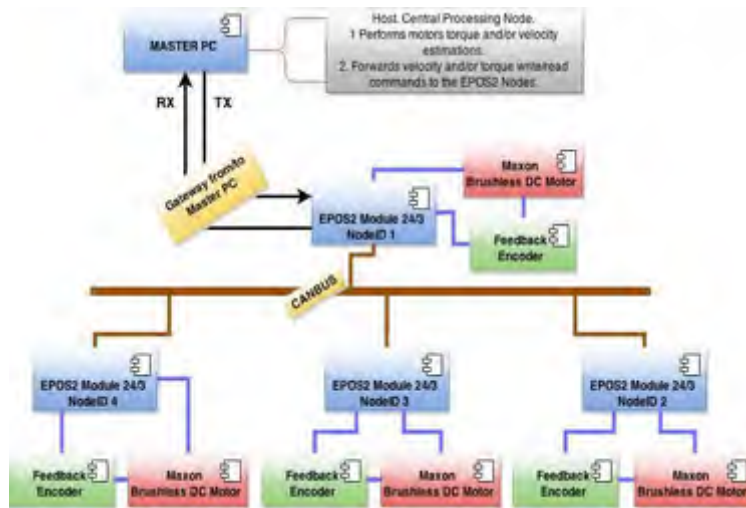
Fig. 16 Architecture of the platform main motion control
