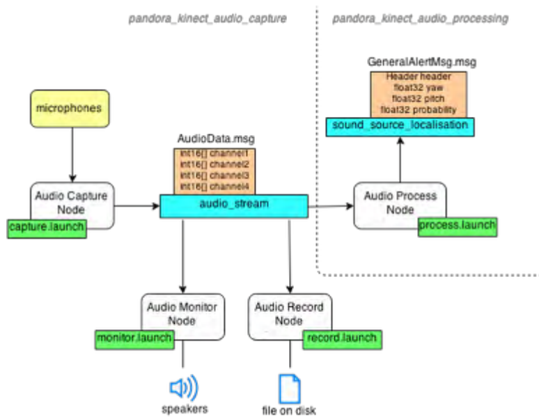
Fig. 14. Audio architecture diagram.
