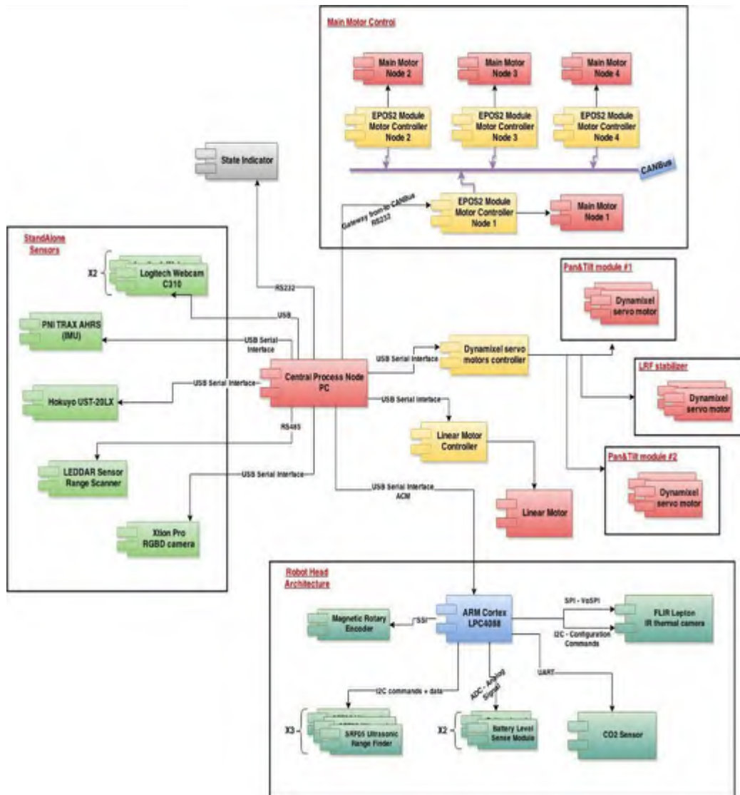
Fig. 4 PANDORA hardware architecture
