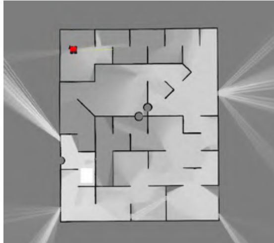
Fig. 5: CRSM SLAM result
