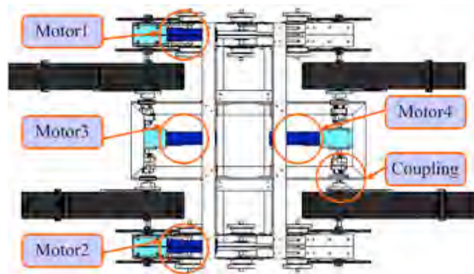
Fig. 8-3. The drive motors configuration
